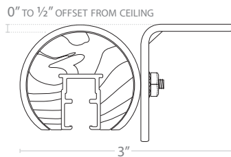
CEILING SUPPORT
